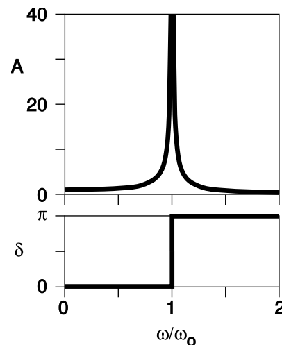
h / Dependence of the amplitude and phase angle on the driving frequency, for an undamped oscillator. The amplitudes were calculated with F_m , m , and \omega_0 , all set to 1.
